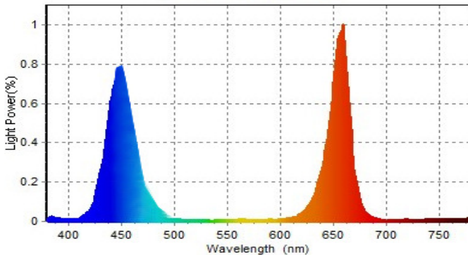
Spectral Distribution Curve
