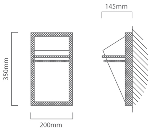
B134 CAD DIAGRAM
