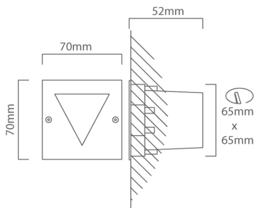
B159 CAD DIAGRAM
