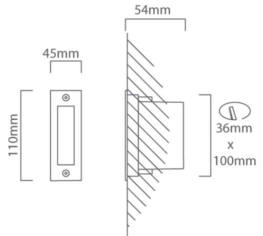
B162 CAD DIAGRAM
