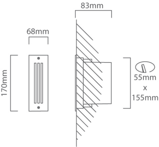
B165 CAD DIAGRAM
