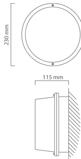
B177 CAD DIAGRAM
