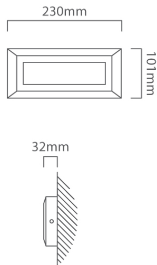
B293 CAD DIAGRAM
