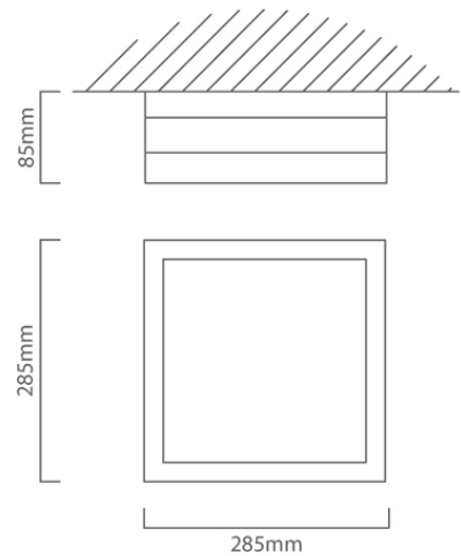
C340 CAD DIAGRAM
