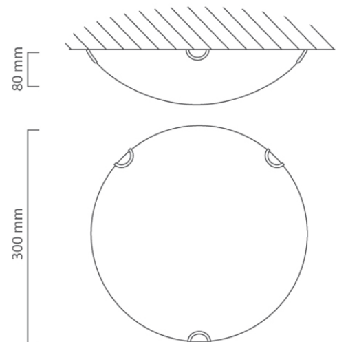
C398 CAD DIAGRAM
