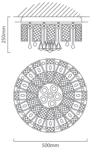
C414 CAD DIAGRAM
