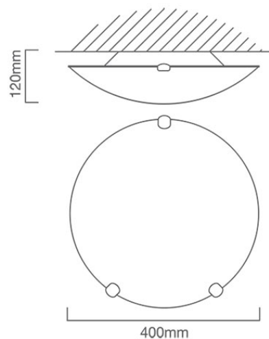
C49 CAD DIAGRAM
