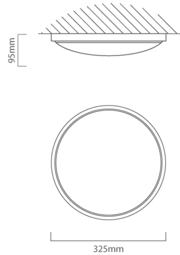
C553 CAD DIAGRAM
