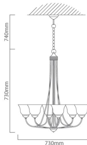
CH110 CAD DIAGRAM
