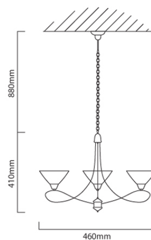
CH192 CAD DIAGRAM
