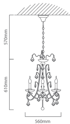
CH217 CAD DIAGRAM
