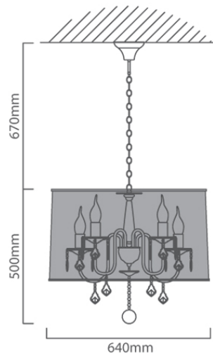
CH228 CAD DIAGRAM
