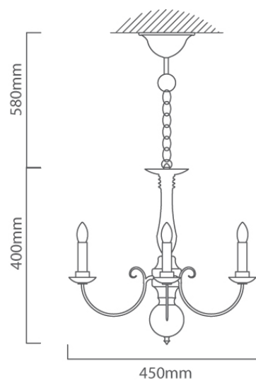
CH4 CAD DIAGRAM
