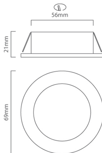
D32 CAD DIAGRAM
