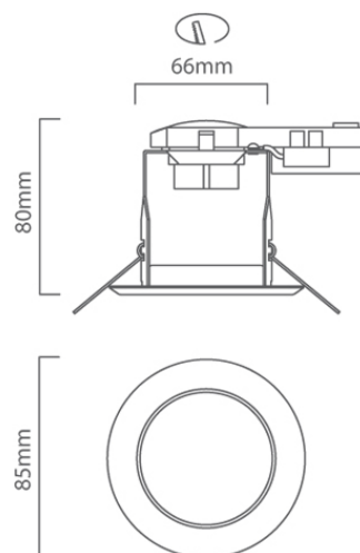
D36 CAD DIAGRAM
