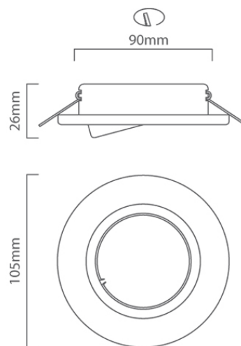
D39 CAD DIAGRAM
