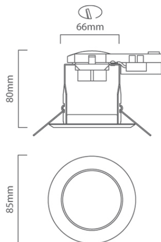
D45 CAD DIAGRAM
