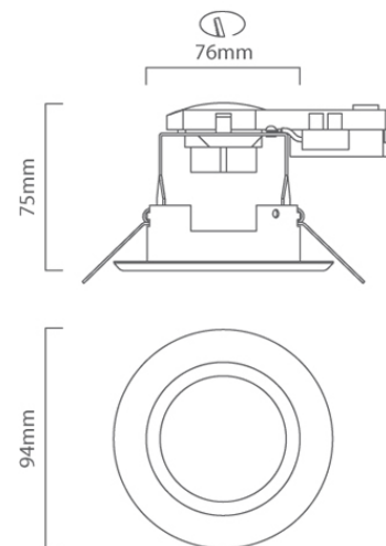
D46 CAD DIAGRAM
