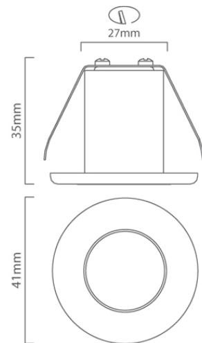
D49 CAD DIAGRAM
