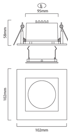
D57 CAD DIAGRAM
