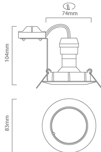
D62 CAD DIAGRAM
