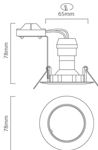
D63 CAD DIAGRAM
