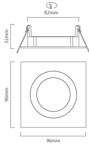
D66 CAD DIAGRAM
