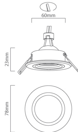
D68 CAD DIAGRAM
