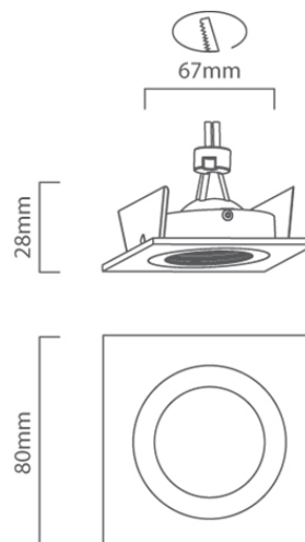
D70 CAD DIAGRAM
