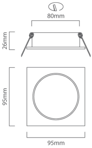
D74 CAD DIAGRAM
