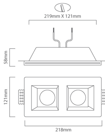
D98 CAD DIAGRAM
