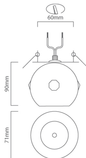
D99 CAD DIAGRAM
