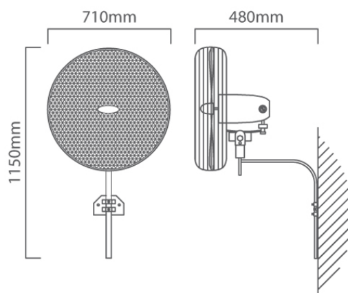
F28 CAD DIAGRAM
