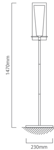
FL113 CAD DIAGRAM
