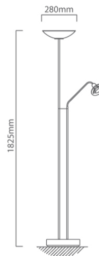
FL12 CAD DIAGRAM
