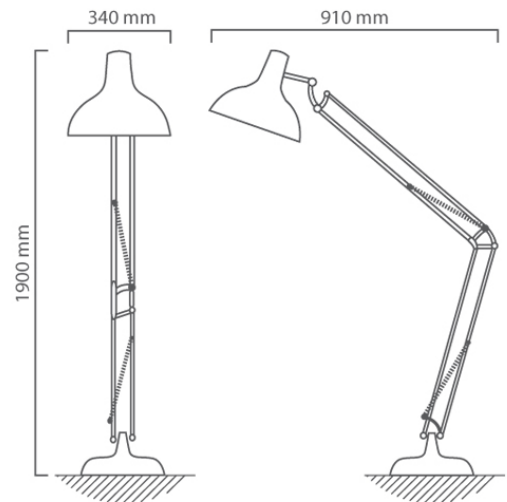
FL188 CAD DIAGRAM
