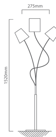
FL21 CAD DIAGRAM
