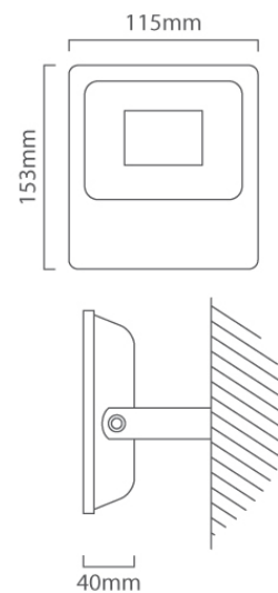
FS171 CAD DIAGRAM
