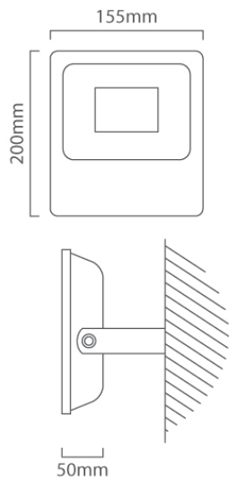
FS172 CAD DIAGRAM
