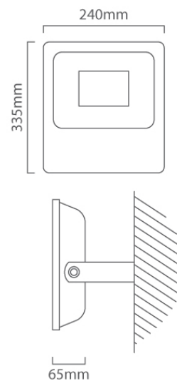
FS173 CAD DIAGRAM
