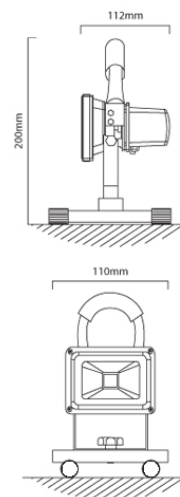
FS203 CAD DIAGRAM
