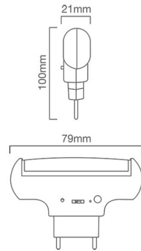
FS211 CAD DIAGRAM
