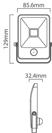
FS255 CAD DIAGRAM
