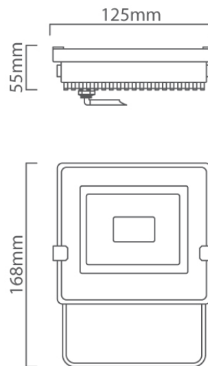
FS260 CAD DIAGRAM
