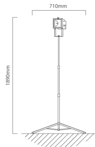
FS3 CAD DIAGRAM
