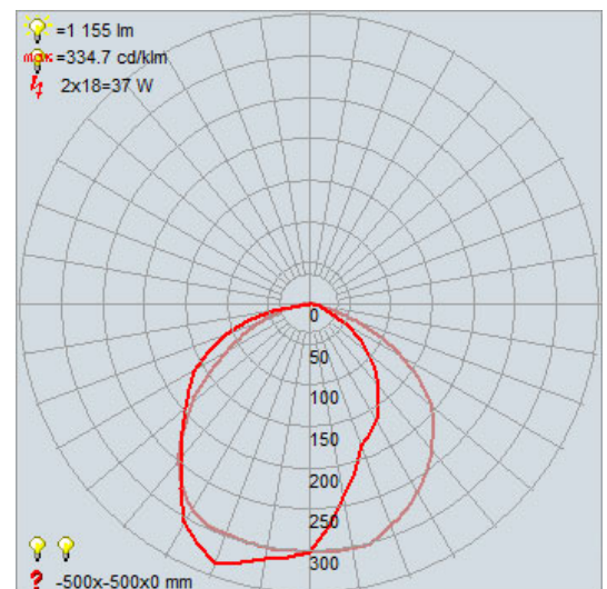
FS3 IES DIAGRAM
