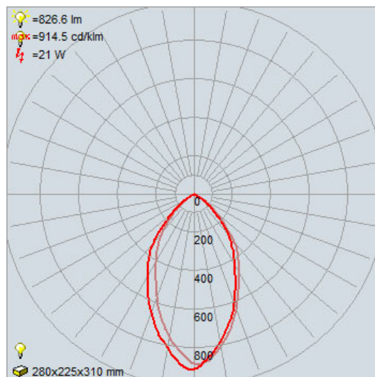
FS9 IES DIAGRAM
