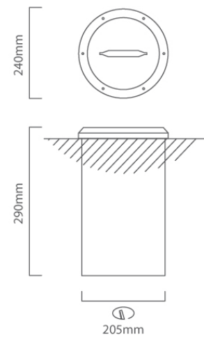
O124 CAD DIAGRAM
