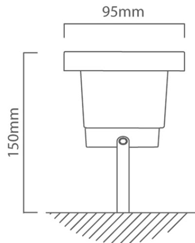
O23 CAD DIAGRAM
