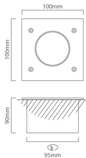
O344 CAD DIAGRAM
