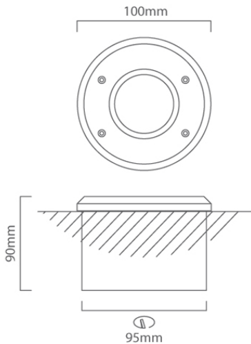
O345 CAD DIAGRAM
